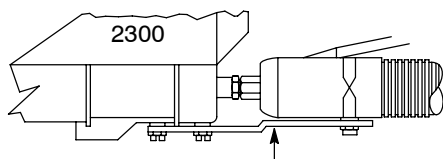
Bracket Kit for 2300 Melters P/N 276318
